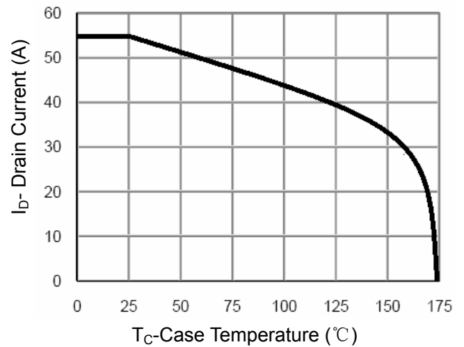
Tc-Case Temperature (°C) Figure 10 Current De-rating
